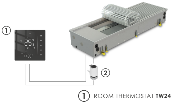
CONNECTION OF ONE FCHV TO ROOM THERMOSTAT
